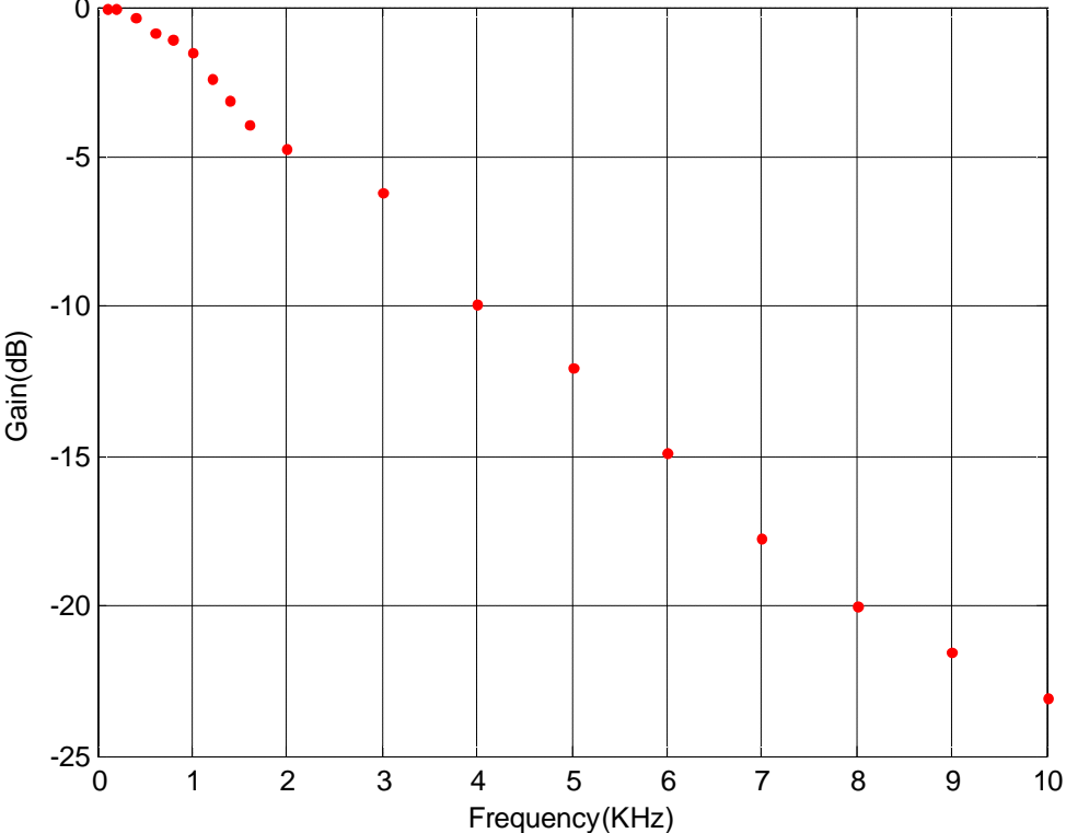
Graph between Gain and Frequency
