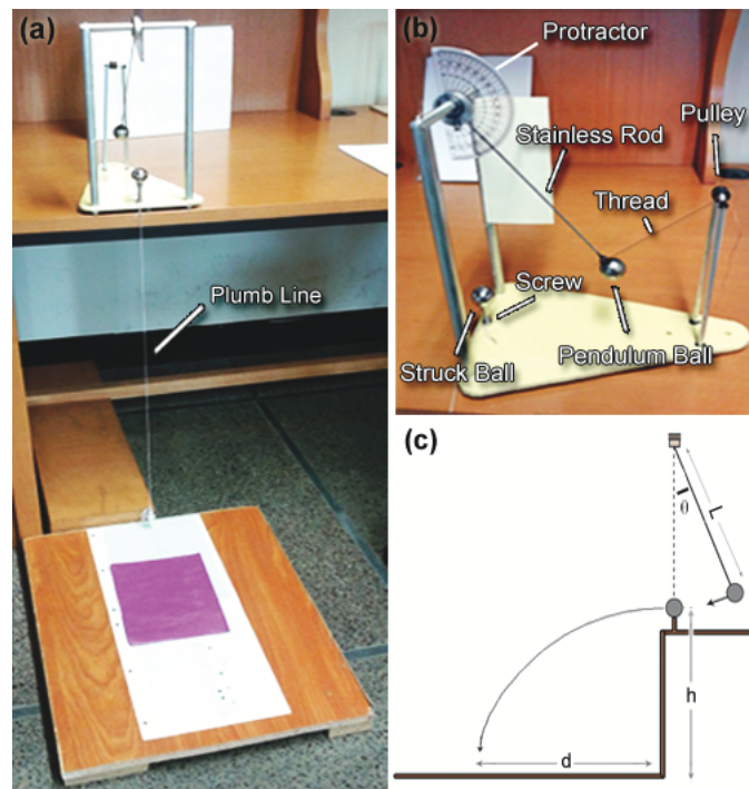
Figure 1: (a) The Experimental Setup; (b) labelled side view of the pendulum and struck ball; (c) illustration of quantities: The length of the pendulum L ; height of collision point h ; angle from the vertical \theta ; horizontal distance from plumb ball d
