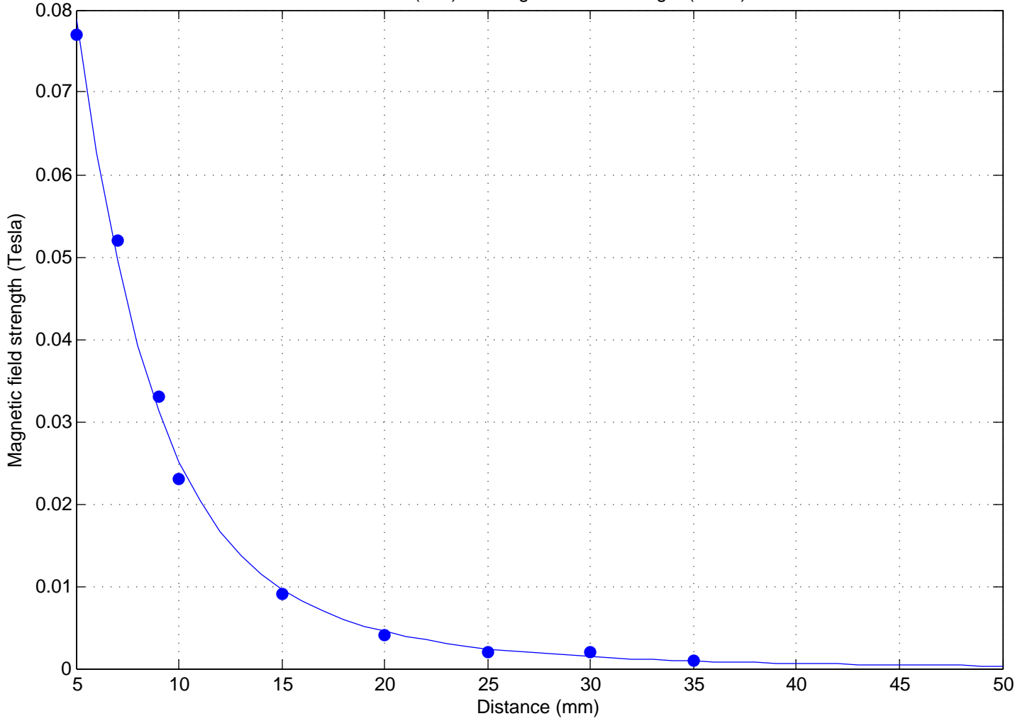
Distance (mm) vs. magnetic field strength (Tesla)
