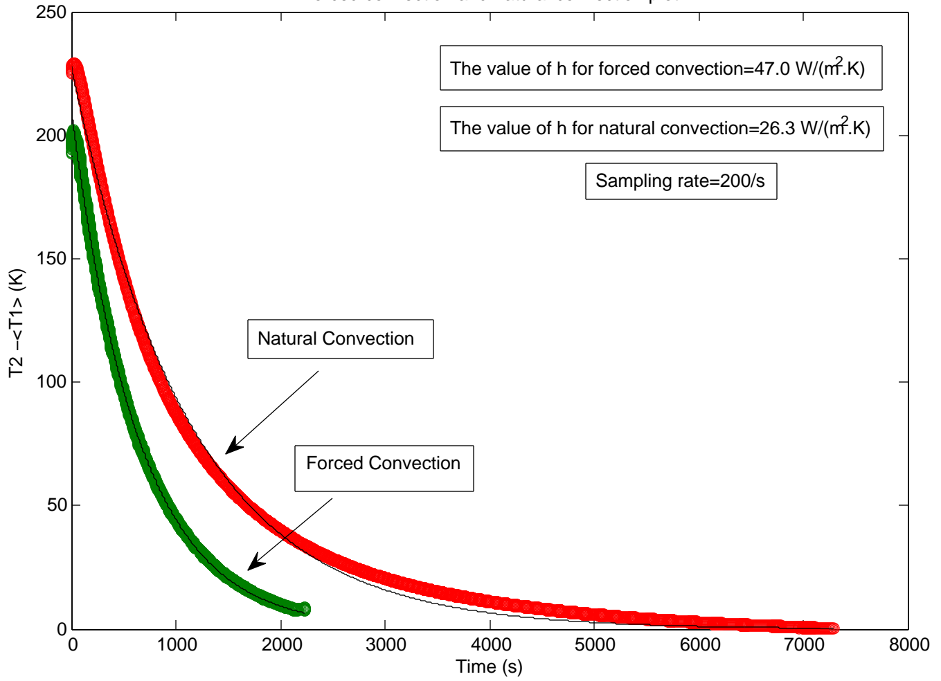
Forced convection and natural convection plot
