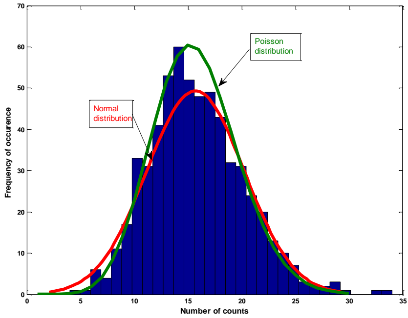
Histogram 10-20 minutes with Gamma source
