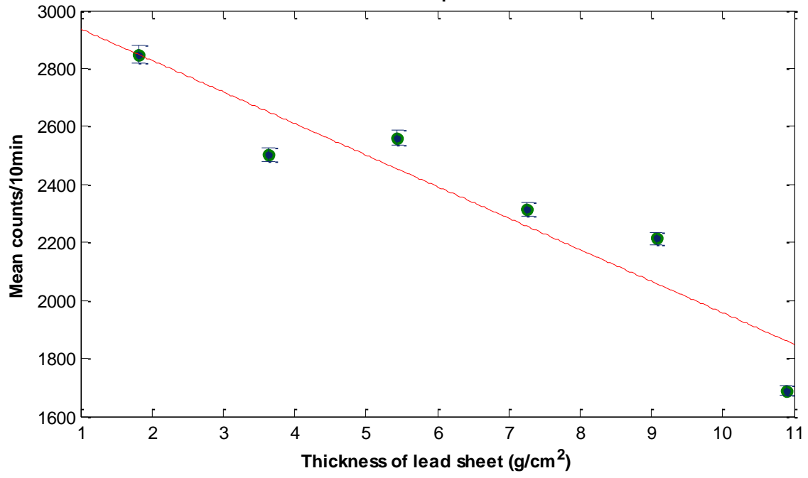
Counts versus thickness plot for Gamma source
