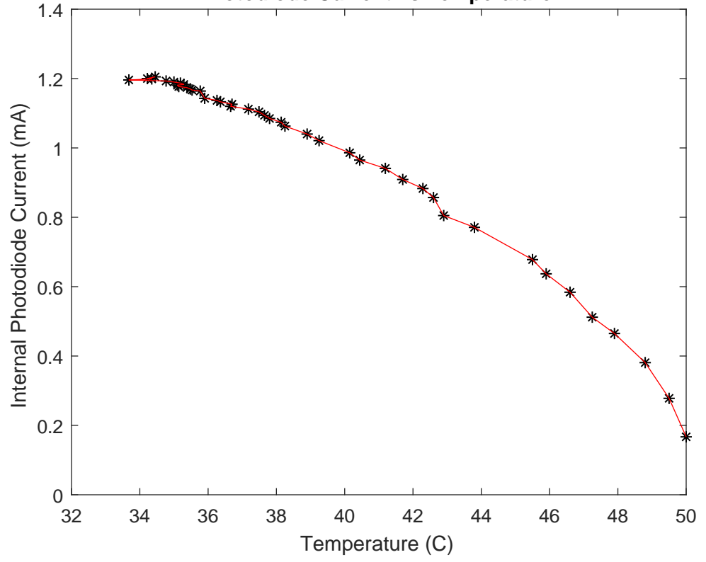
Photodiode Current vs Temperature
