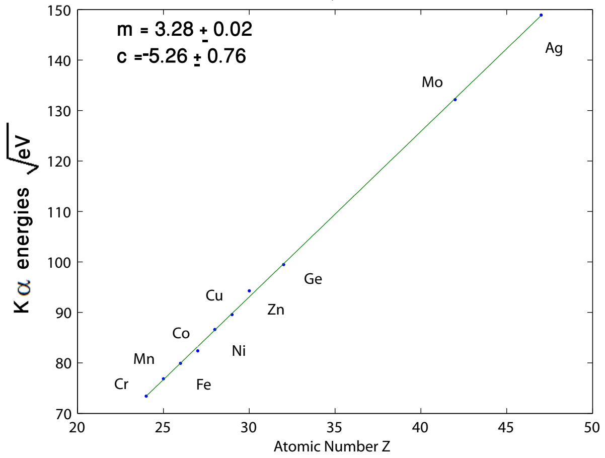
Moseley's Law
