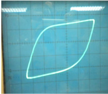
Ferroelectric loop at 130°C
