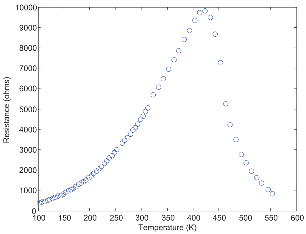
Resistance versus temperature plot of UJT
