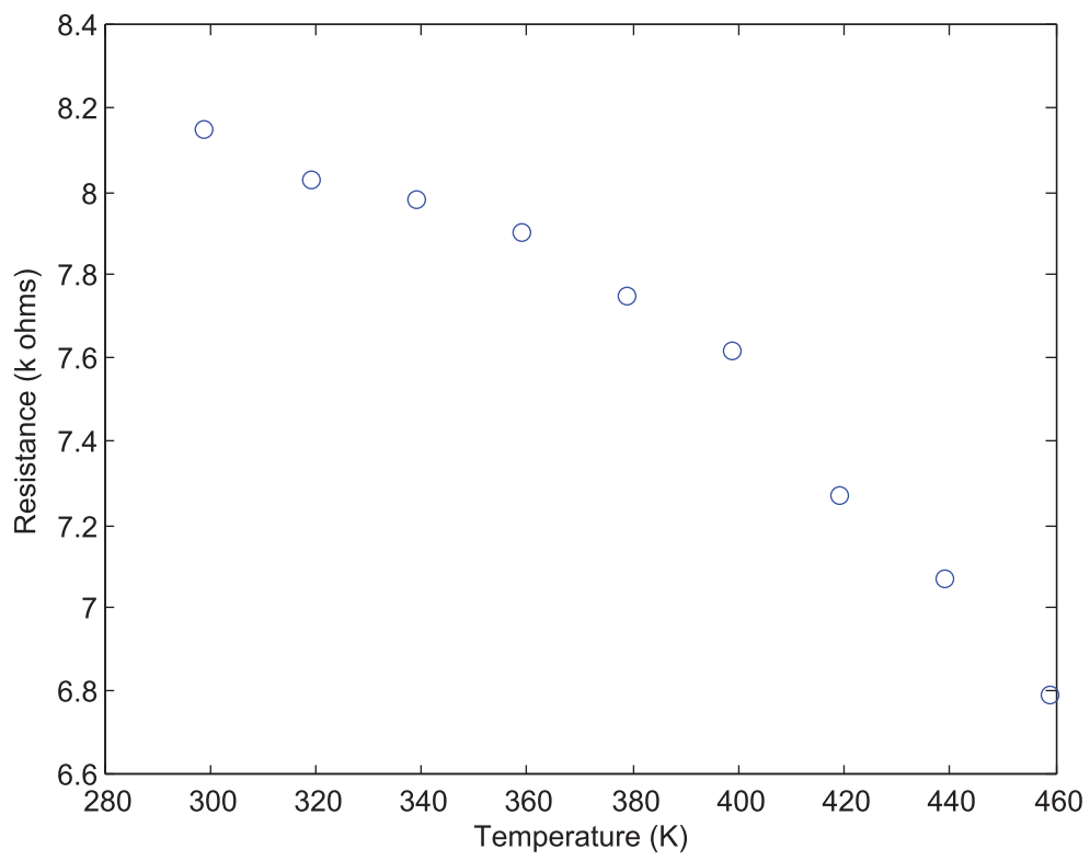
Resistance versus temperature plot of carbon resistor
