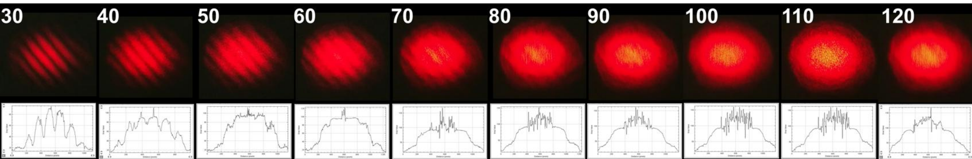
The interference patterns as P3 rotates, corresponding to the setup of Figure 4.
