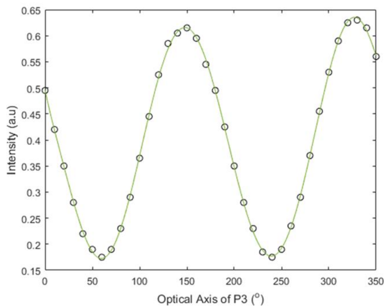
Optical intensity as P3 rotates. (corresponding to the setup of Figure 4.)
