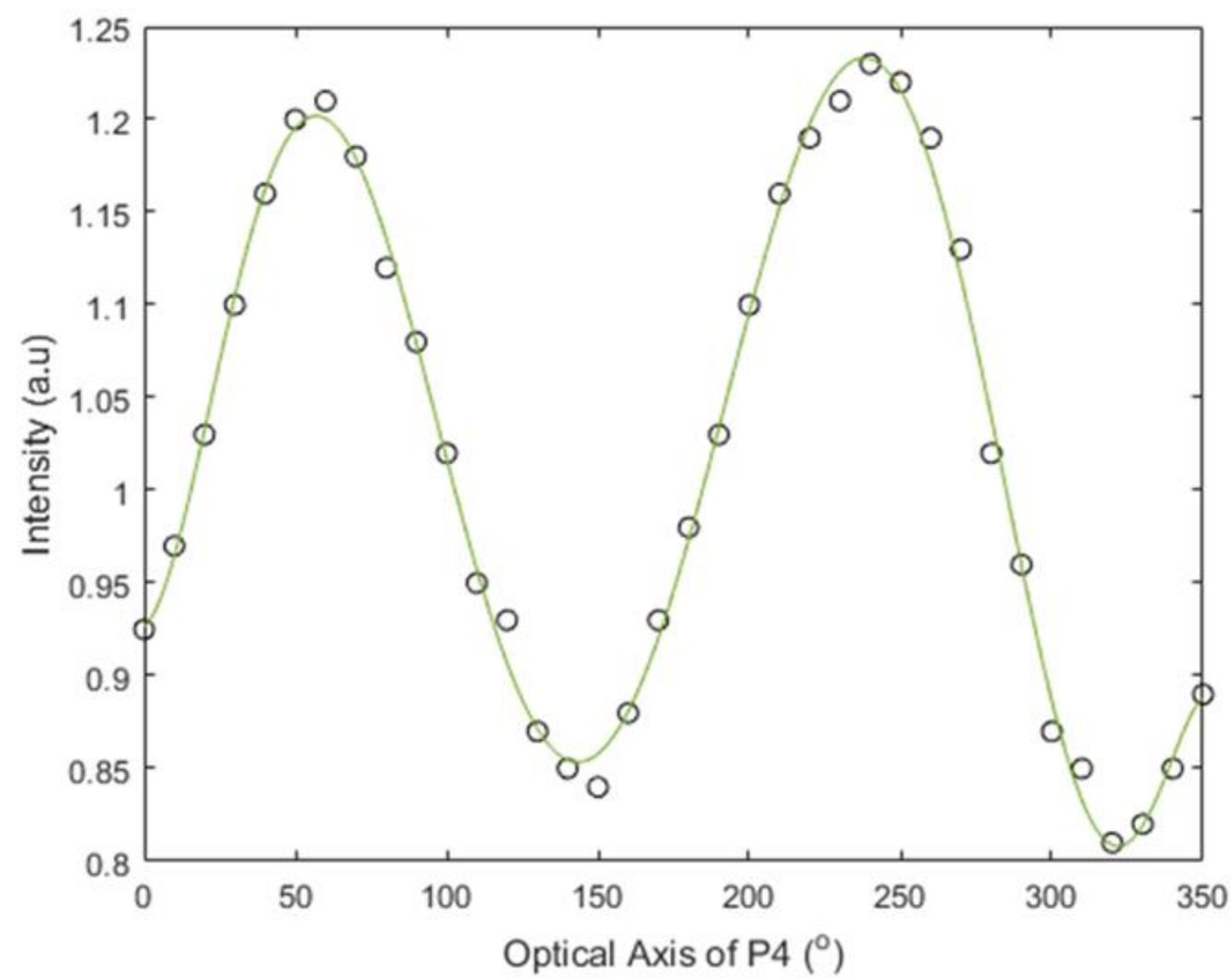
Optical intensity as P4 rotates. (corresponding to the setup of Figure 5.)
