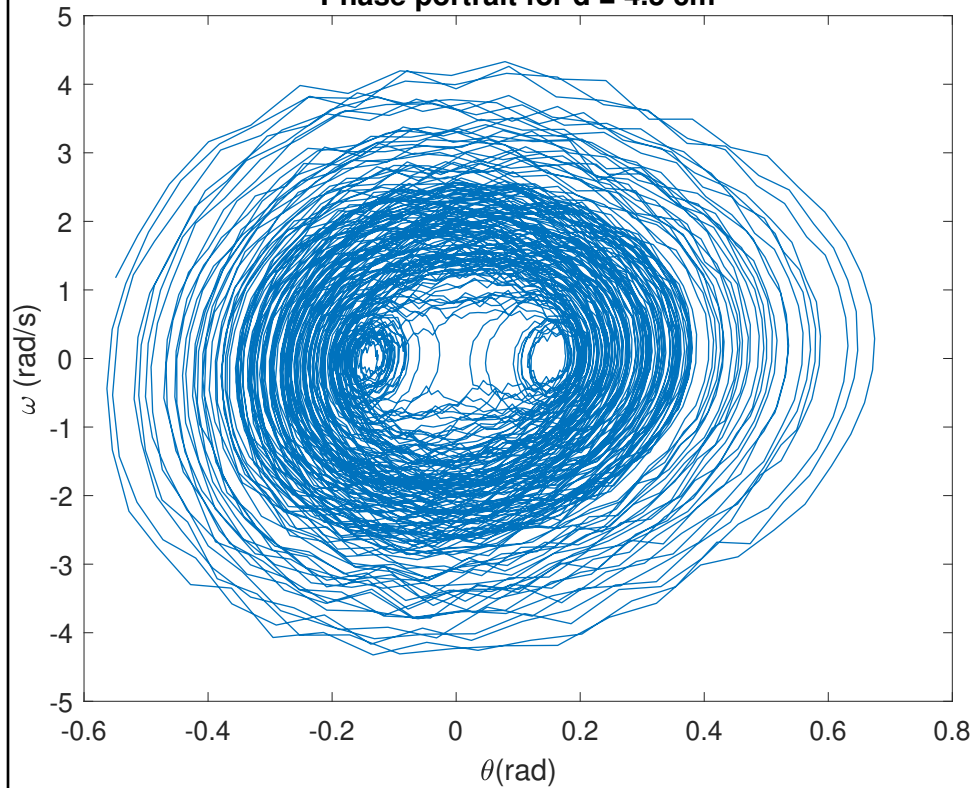
Phase portrait for d = 4.5 cm
