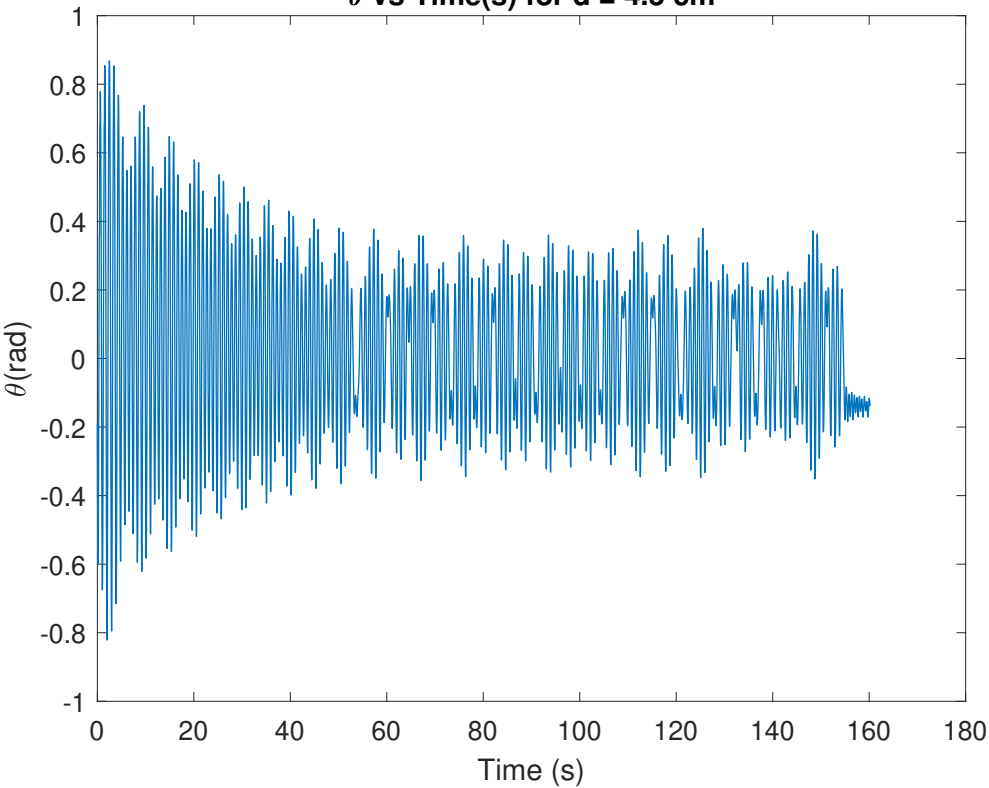
\theta vs Time(s) for d = 4.5 cm
