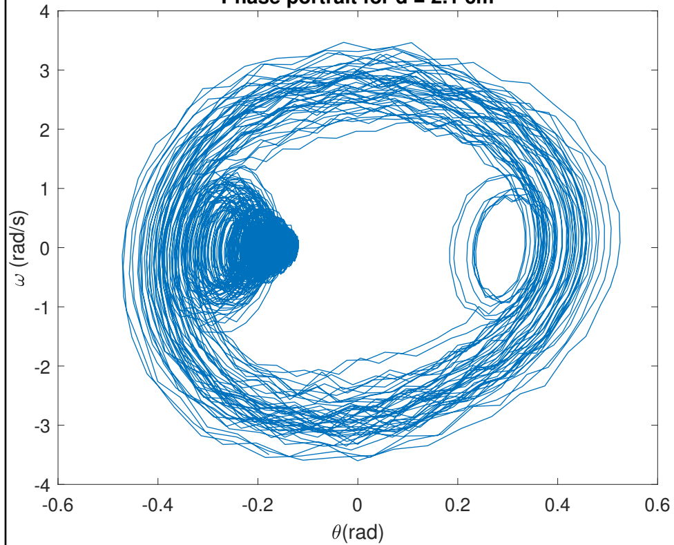
Phase portrait for d = 2.1 cm
