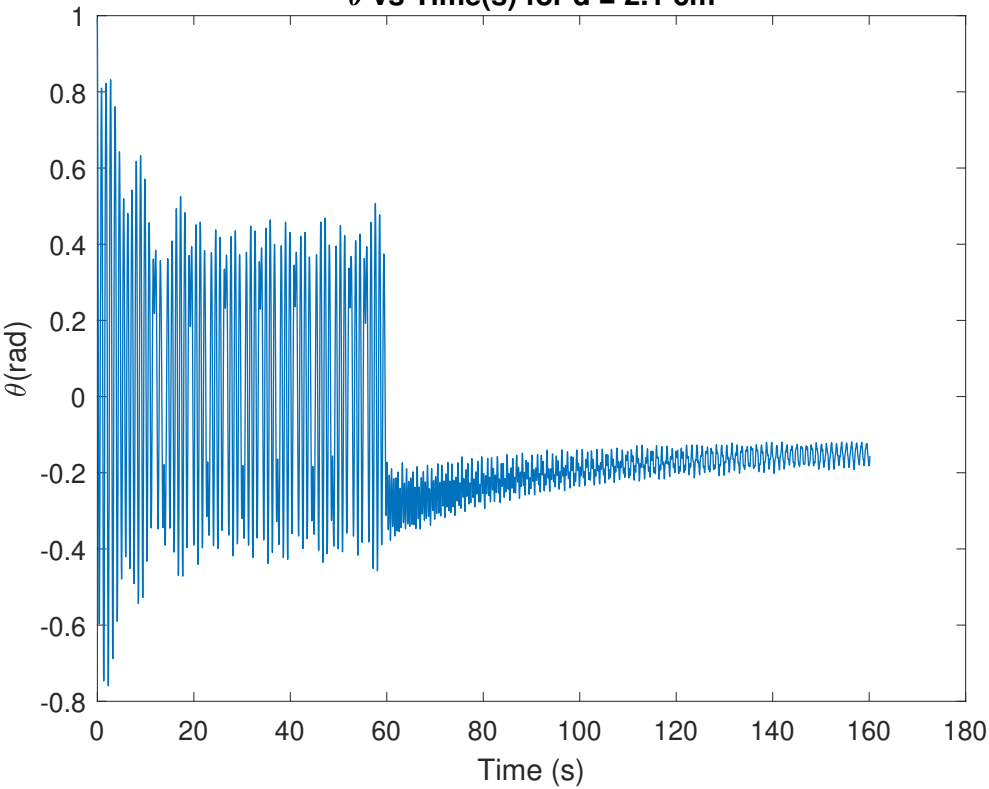
\theta vs Time(s) for d = 2.1 cm
