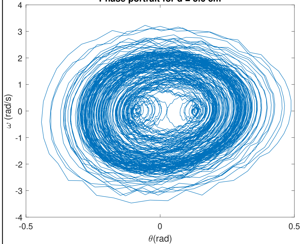
Phase portrait for d = 5.6 cm
