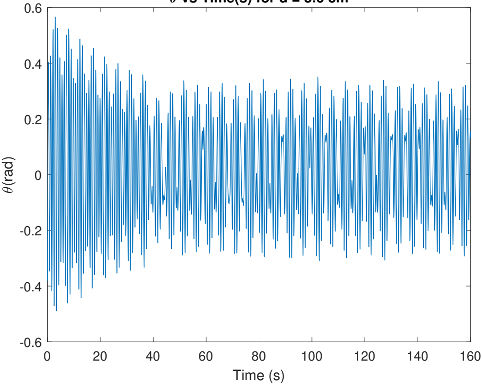
\theta vs Time(s) for d = 5.6 cm
